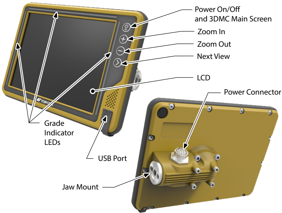
Figure 1: GX-55/GX-75 Display – Front and Rear View
